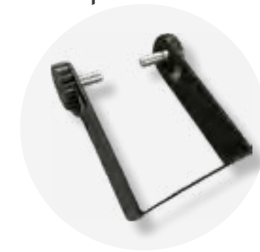
SECTIONAL CONNECTORS
