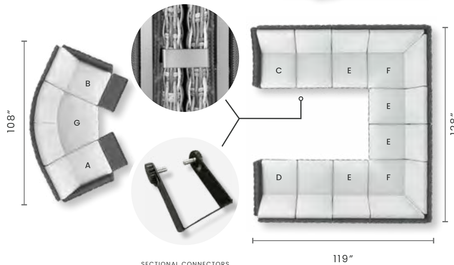
SECTIONAL CONNECTORS
